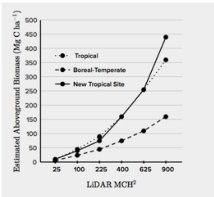
Carbon Biomass and Mean Canopy Height (MCH) in Different Types of Forests
